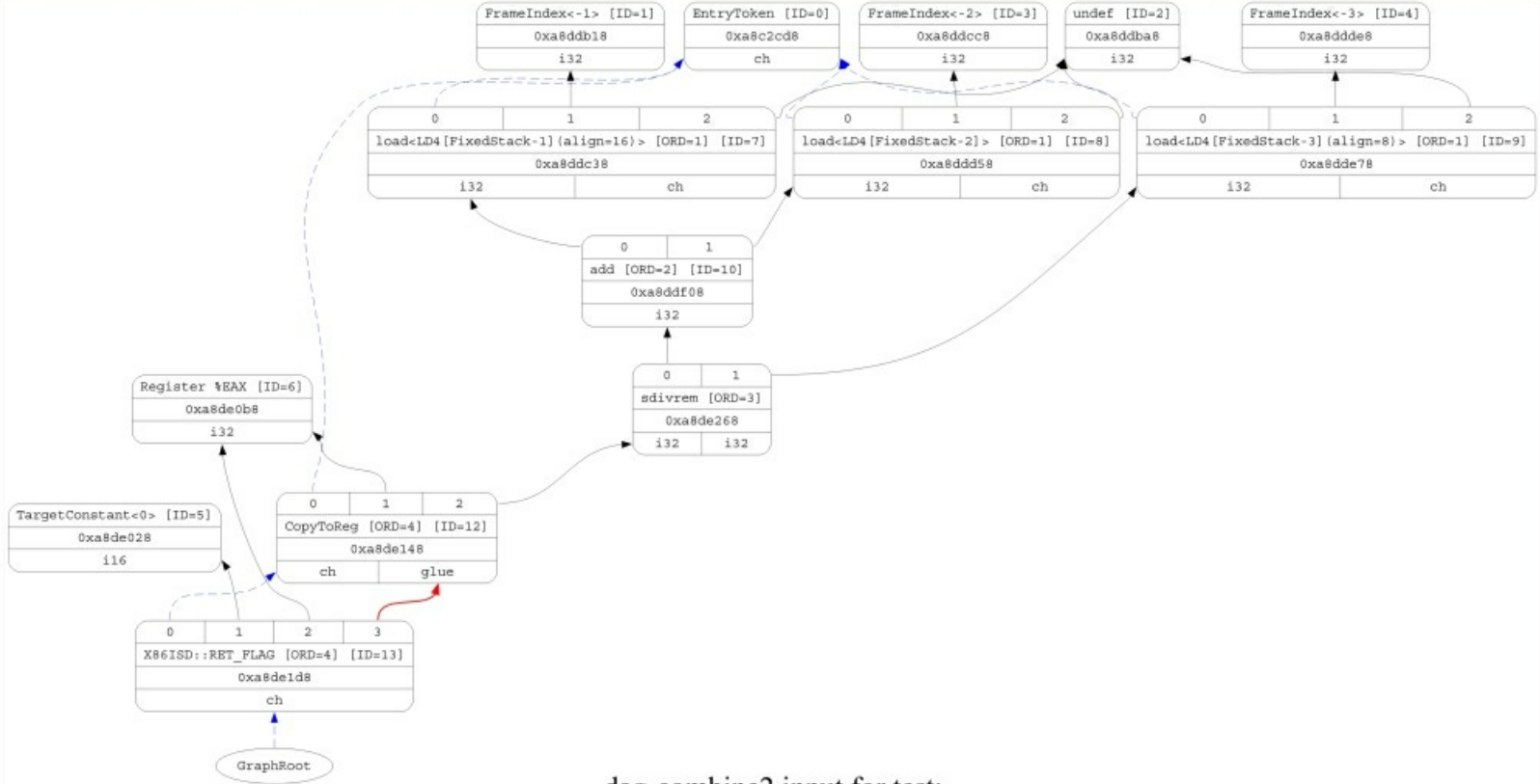
dag-combine2 input for test:
