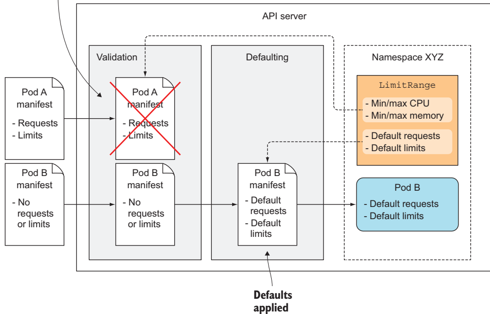
Figure 14.6 A LimitRange is used for validation and defaulting pods.
