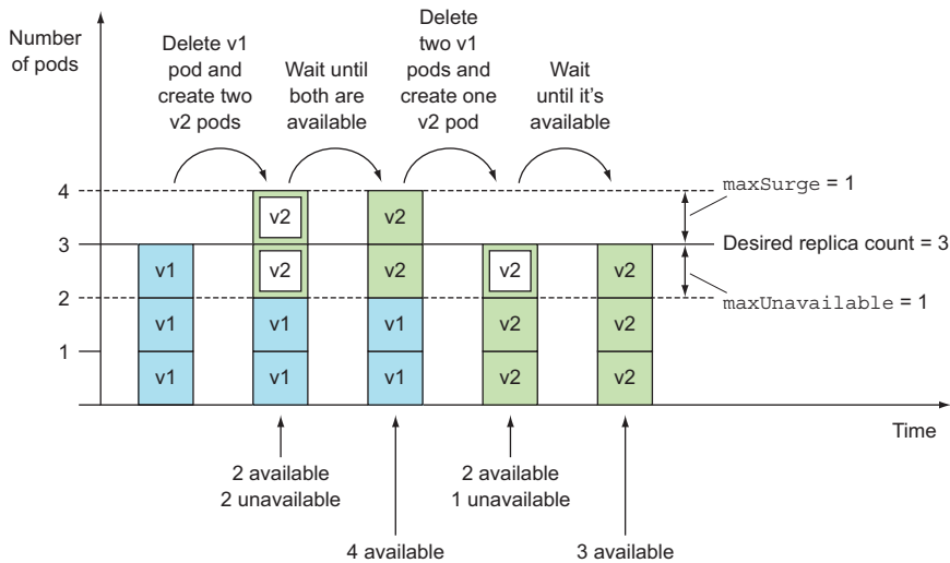
Figure 9.13 Rolling update of a Deployment with the \text{maxSurge} = 1 and \text{maxUnavailable} = 1
